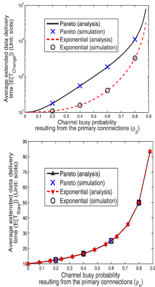
Fig (2) and (3) Effects of Pareto and exponential service time distributions for Primary connections on the extended data delivery time ( E[T]_{change} ) and ( E[T]_{stay} ).
